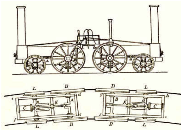
The "South Carolina," 1831, and plan of its running gear.
