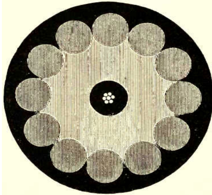
Shore End of Cable-exact size. [About 3.5 inches in diameter.]
