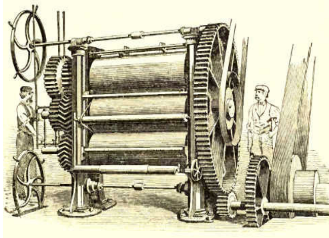
Calenders heated internally by Steam, for spreading India Rubber into Sheets or upon Cloth, called the "Chaffee Machine."
