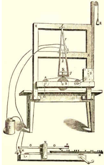
The First Telegraphic Instrument, as exhibited in 1837 by Morse.
