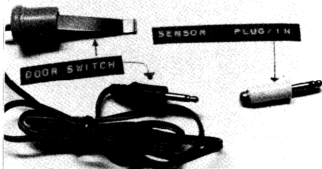
Photo 2. The completed sensor plug in unit and the door-switch unit it replaces.
