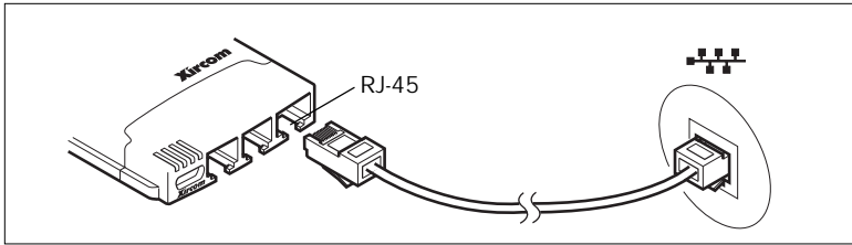
Connecting to a 100Base-TX or 10Base-T LAN (RJ-45)
