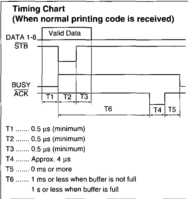
Timing Diagram
