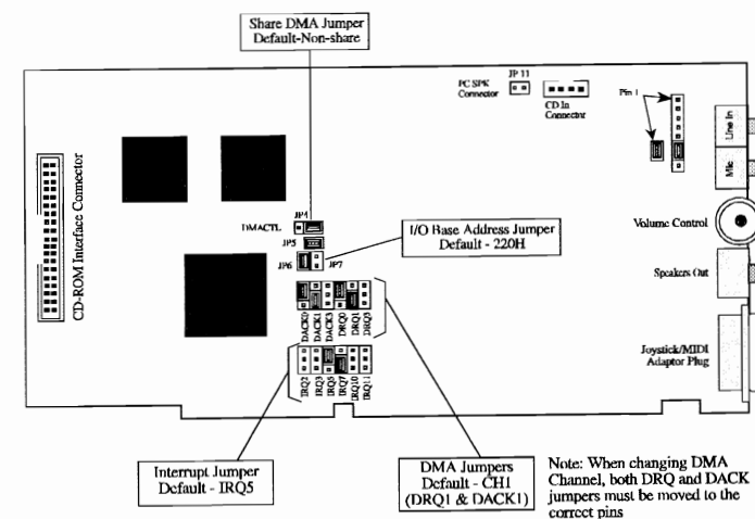
Figure B-1: Jumpers on the audio card.
